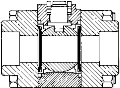
Ball valve
