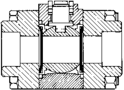
Ball valve
