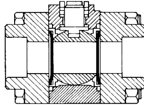
Ball valve
